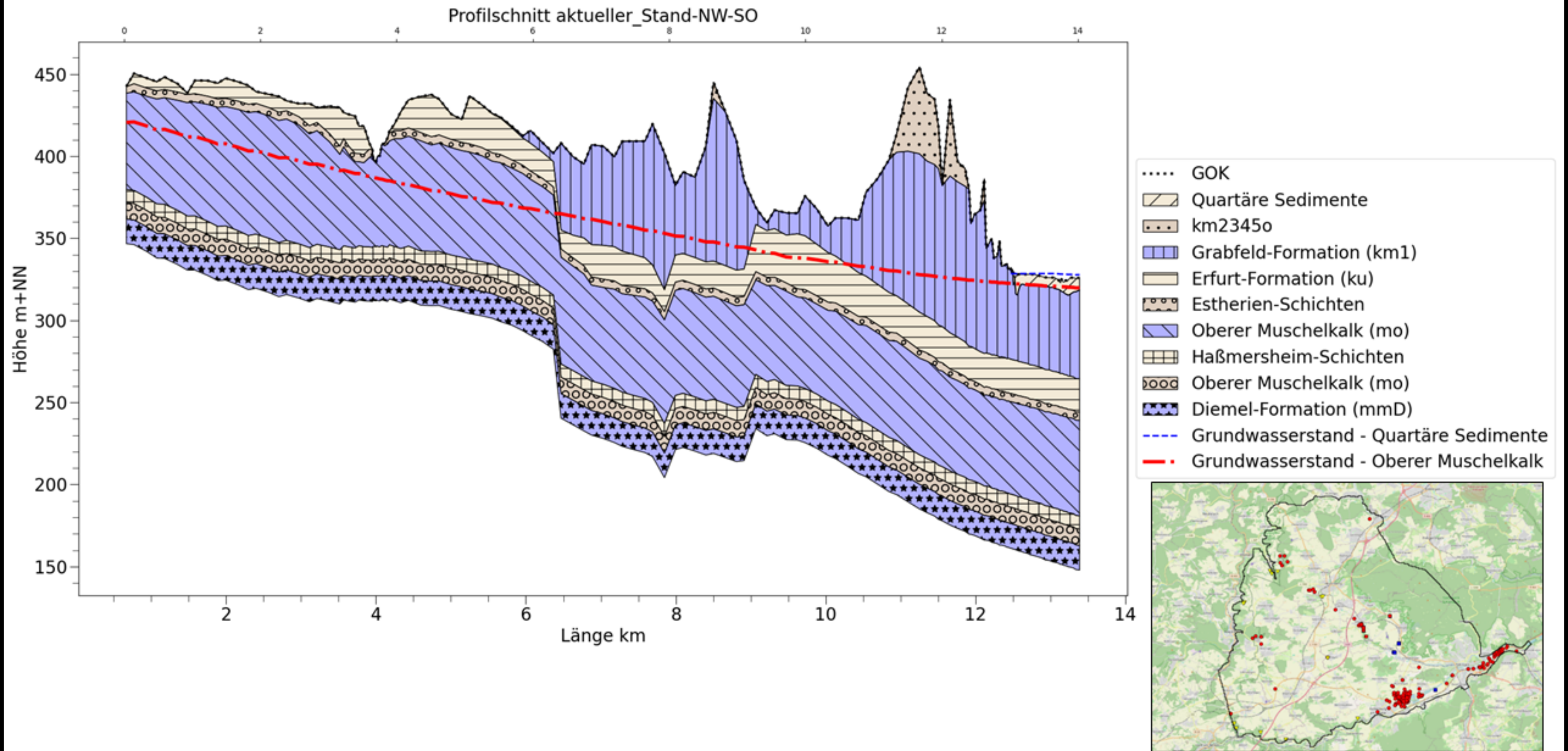
A cross-section of the geological layers in the groundwater model
