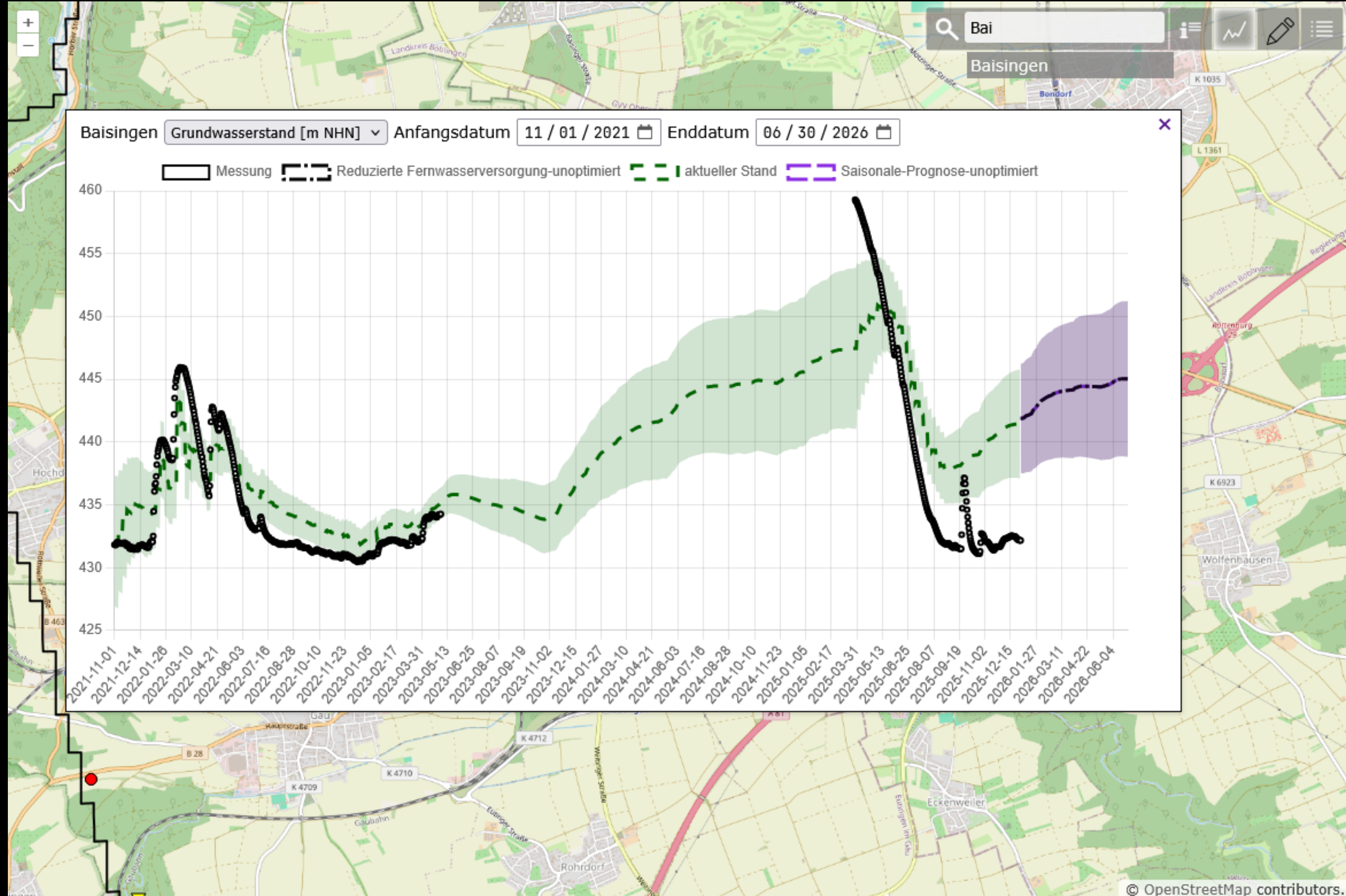
The measured and simulated groundwater level at a monitoring site
